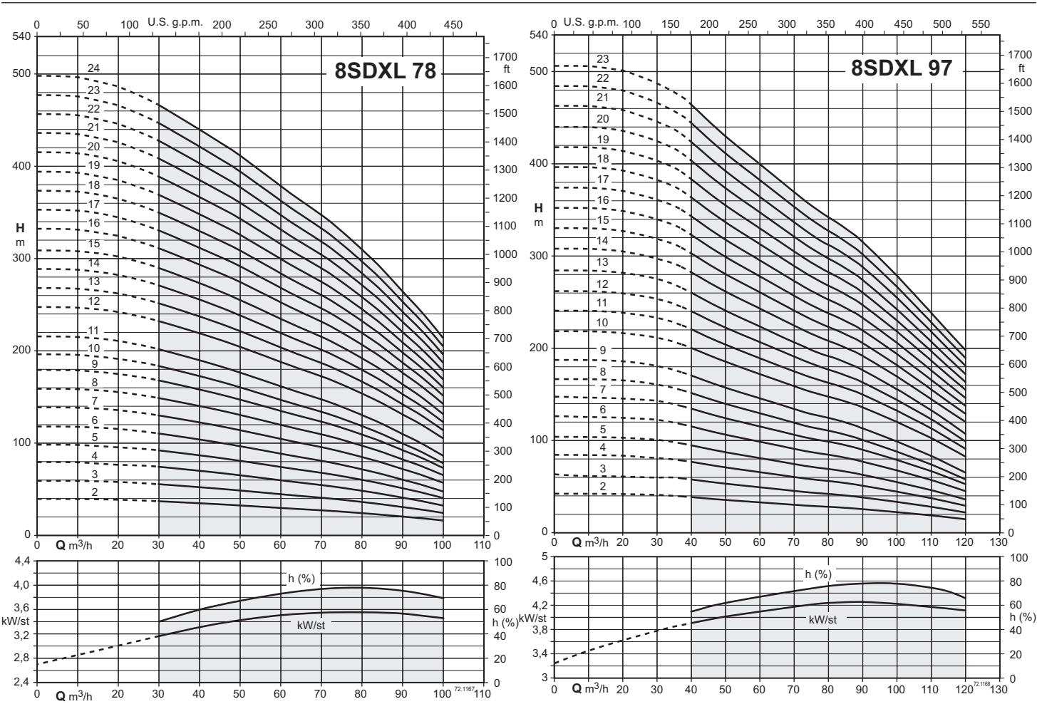
Coverage chart n ≈ 2900 rpm
