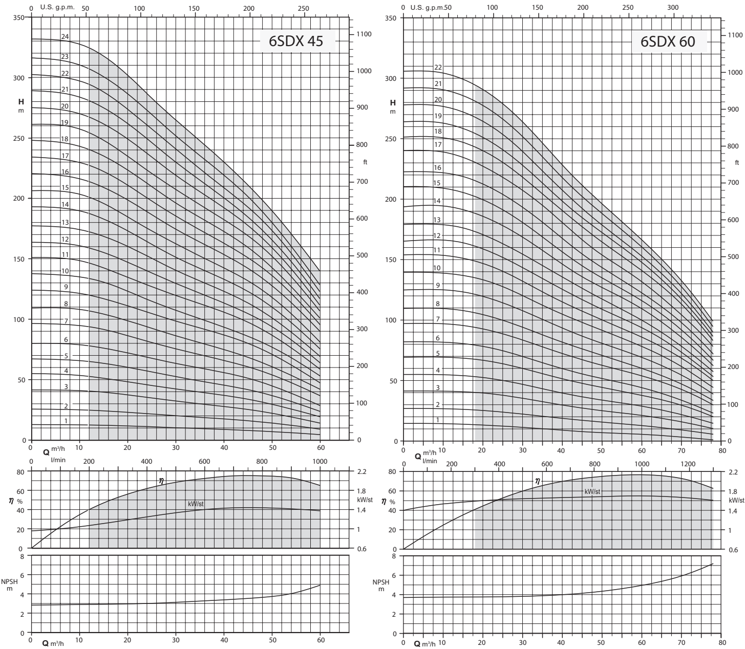
Coverage chart n ≈ 2900 rpm
