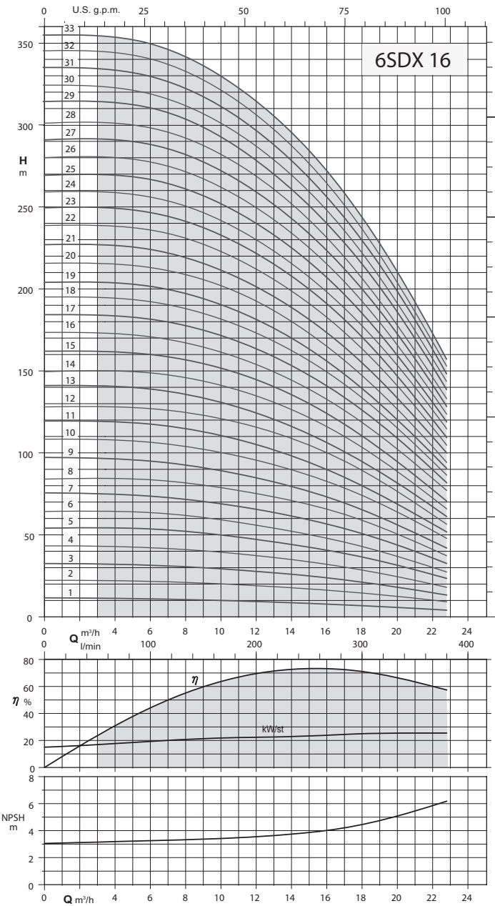
Coverage chart n ≈ 2900 rpm
